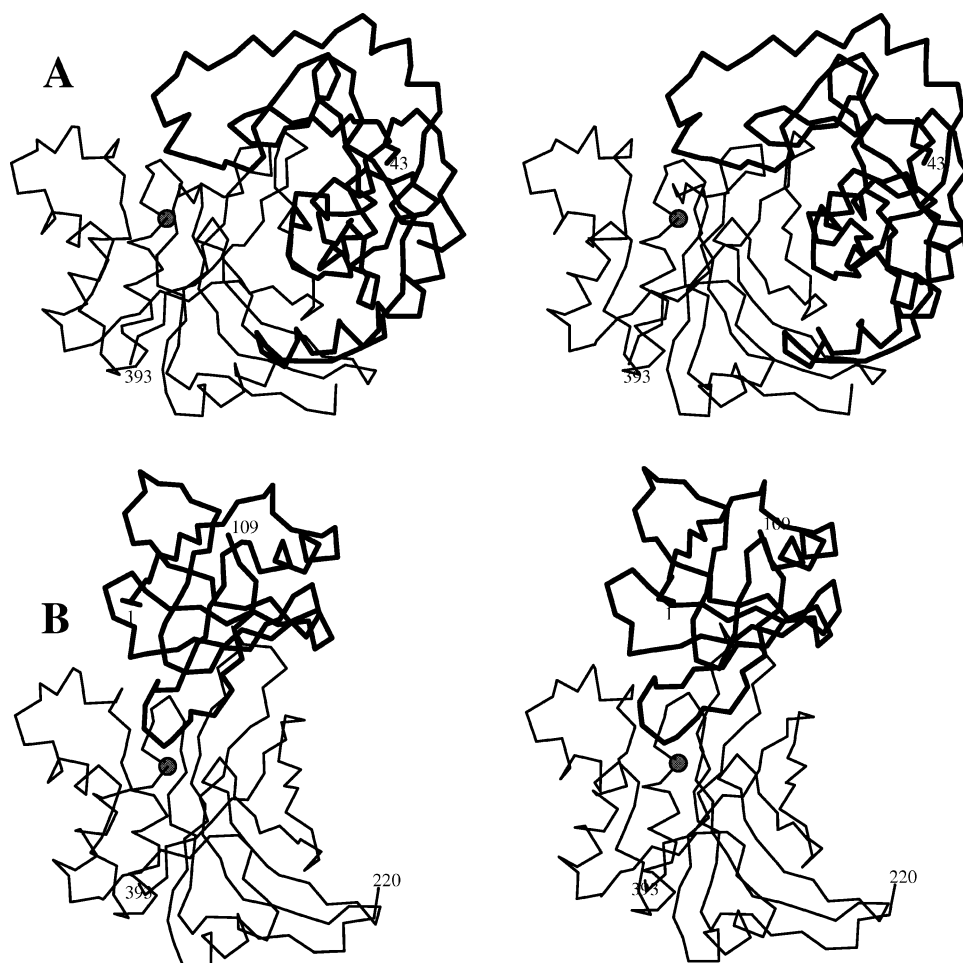
FIGURE 5: Stereo C \alpha trace of (A) prostaphopain B and (B) the staphopain B–staphostatin B complex. The mature forms of the protease are in analogous orientations in both parts of the figure, and are shown as thin lines. The black balls mark the positions of the C \alpha atoms of the active site cysteines. The prostaphopain B proregion in panel A and staphostatin B in panel B are shown with thick lines. Note that in panel B the black balls mark the positions of the C \alpha atoms of alanine, because this crystal contained the inactive Cys243Ala mutant of the protease.
