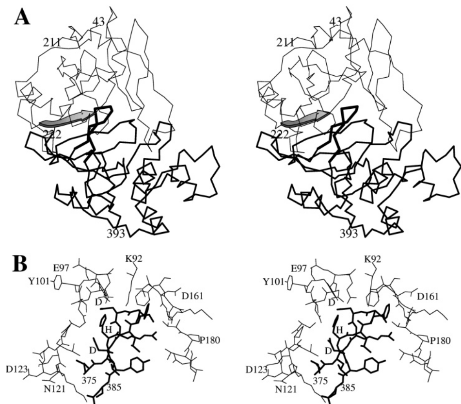
FIGURE 2: Stereodiagrams of the interactions between the proregion of prostaphopain B (thin lines) and the mature form (thick lines). (A) C^\alpha trace of prostaphopain B. The edge strand of the proregion that interacts with an edge strand of the mature form is shown in ribbon representation. The staphopain specific loop that inserts into the half-barrel of the proregion is drawn with extra thick lines. (B) The same loop is shown in the identical orientation in an all-atom representation together with residues of the proregion that are <4 \text{ \AA} from it (and with some bridging residues of the proregion that have been included to reduce the number of polypeptide chain fragments in the drawing). Asp98 of the proregion and His377 and Asp383 of the mature form that form two salt bridges have been labeled in the one-letter convention.
